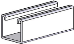
12 GAUGE 1-5/8" x 1-3/8"
