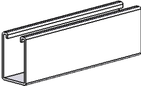
12 GAUGE 1-5/8" x 3-1/4"
