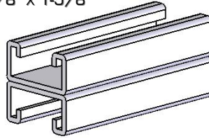
12 GAUGE 1-5/8" x 2-3/4"
